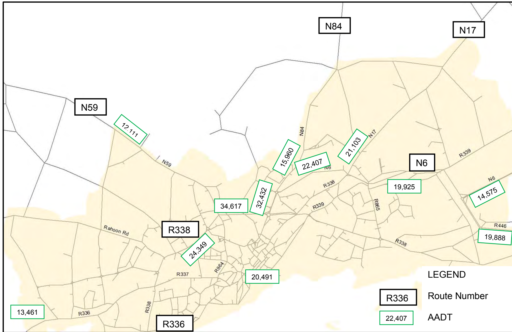
Figure 2.3: Existing Traffic Volumes (AADT)
